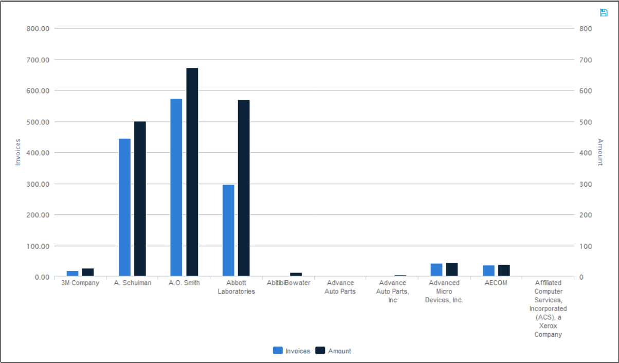
Figure 2.18: Column Chart
